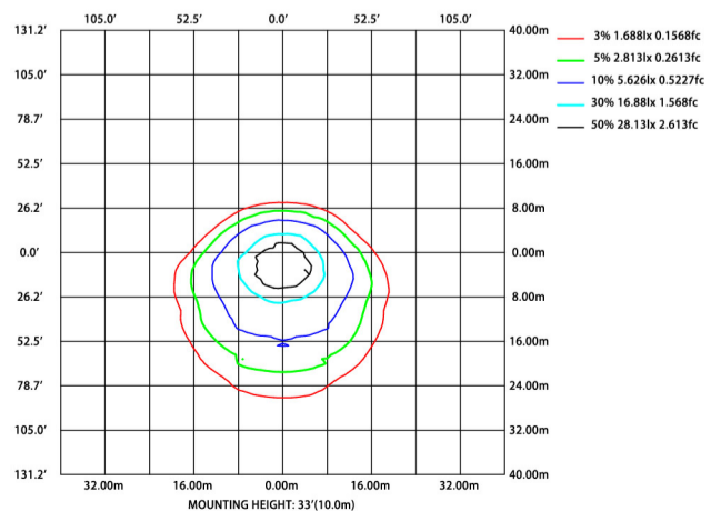
ISOLUX DIAGRAM
