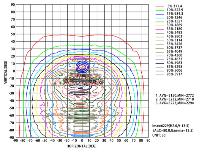
ISOCANDELA DIAGRAM
